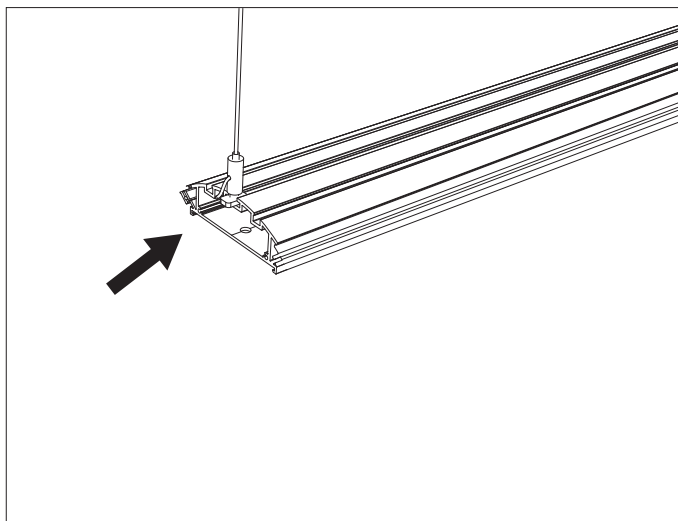
3. Install the suspension kits
